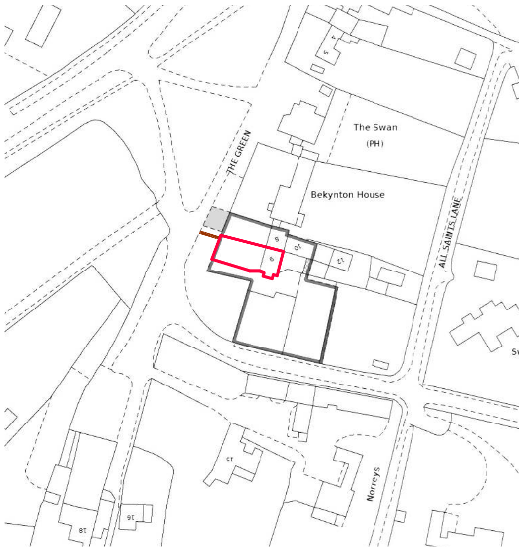
easement plan no 9 the green scale 1-1250
